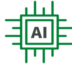
Artificial Intelligence
